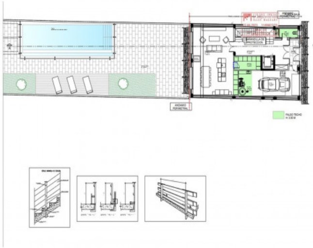
Floor plan
