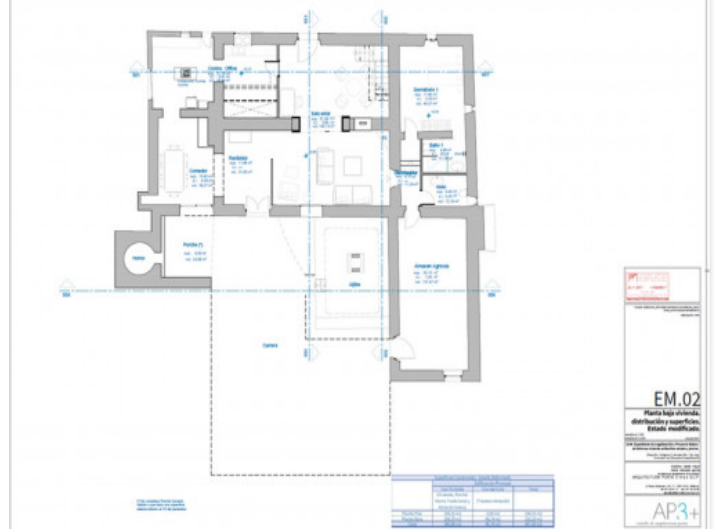
Plan groundfloor
