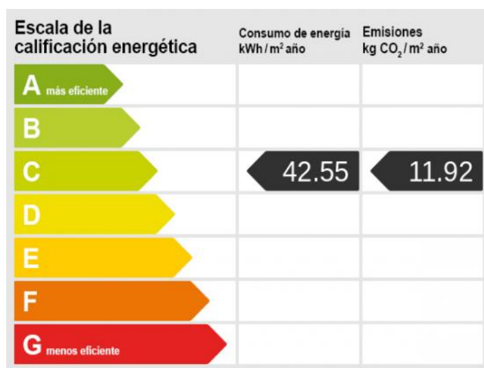
Energy scale
